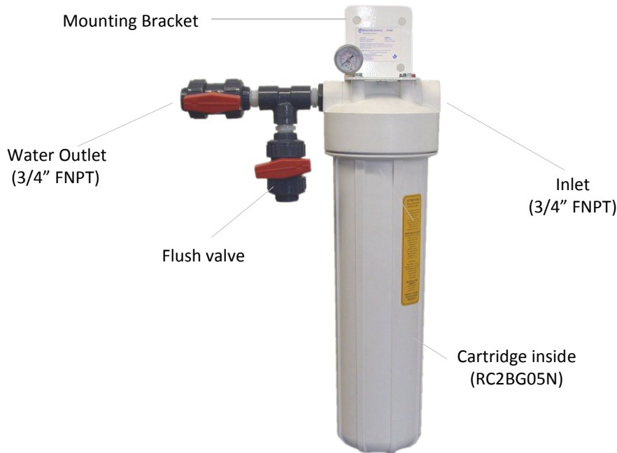
Fig : EG12B Espresso Water Filter System
