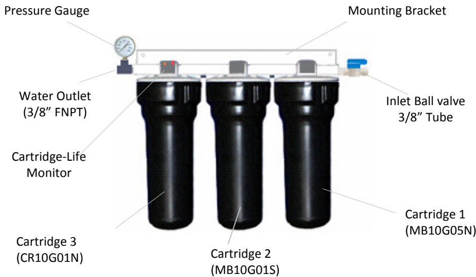
Fig : IG31U Ice Maker Water Filter System
