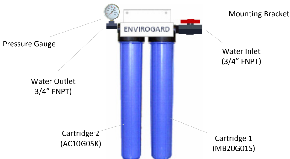
Fig : MG22W Water Filter System for multiple applications
